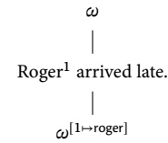
Figure 4: Deterministic update
